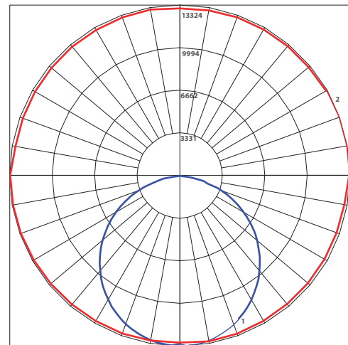
Maximum Candela = 13324.76 Located At Horizontal Angle = 0, Vertical Angle = 2.5 #1 - Vertical Plane Through Horizontal Angles (0-180) (Through Max. Cd.) #2 - Horizontal Cone Through Vertical Angle (2.5) (Through Max. Cd.)
