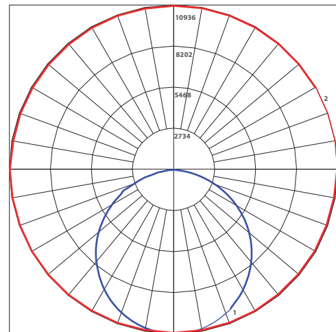
Maximum Candela = 10935.99 Located At Horizontal Angle = 0, Vertical Angle = 2.5 #1 - Vertical Plane Through Horizontal Angles (0-180) (Through Max. Cd.) #2 - Horizontal Cone Through Vertical Angle (2.5) (Through Max. Cd.)
